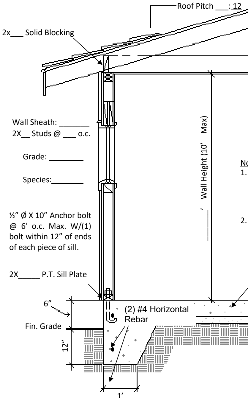
WALL SECTION – MONOLITHIC SLAB
