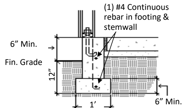
STEMWALL FOOTING
